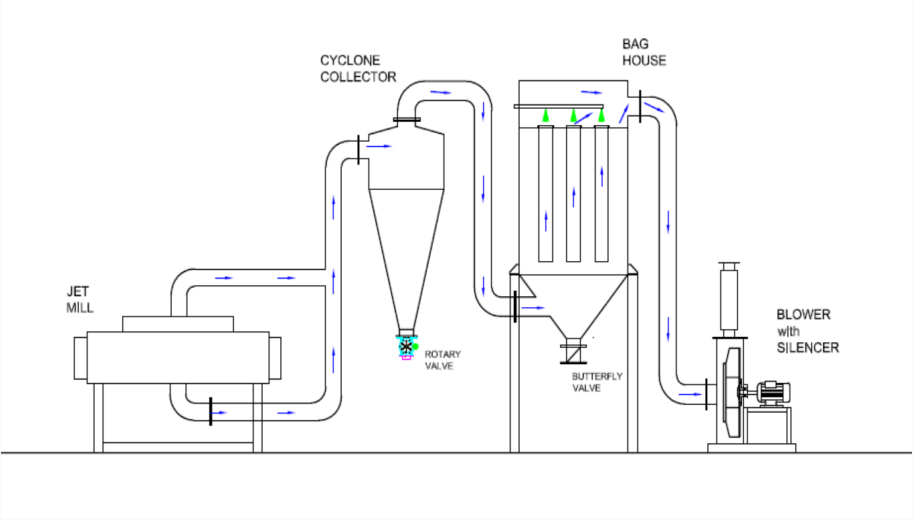
Jet Milling System
