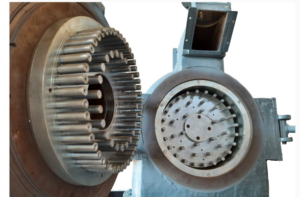
PIN MILL FOR COARSE GRINDING | 800 Kg/hr
