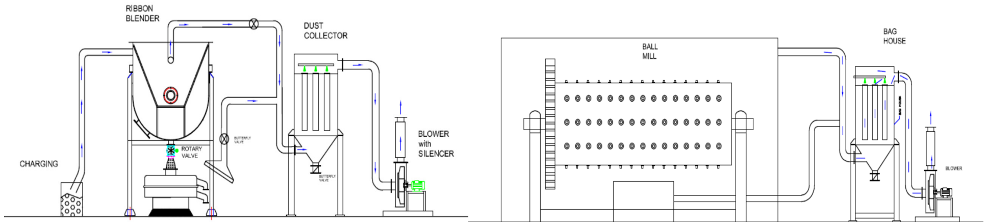
Ribbon Blender System
